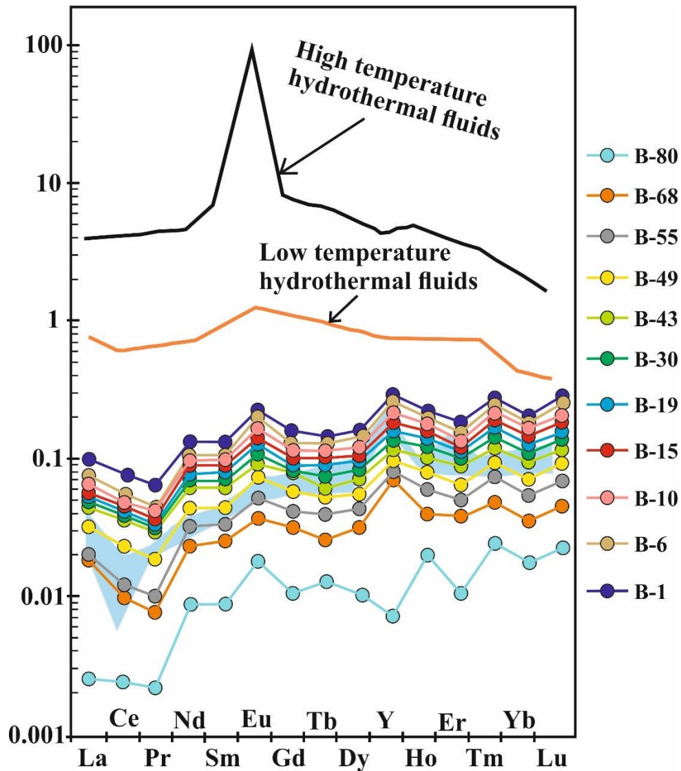
Graph 1. Shale normalized (PAAS) REE+Y diagram of the Saytepe carbonate samples. The blue area denotes present-day seawater
