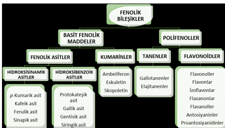
Figure 1.1. Classification of phenolic compounds (Vermerris and Nicholson, 2008).
