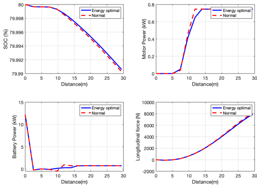
Figure 5. Results of 2.86 ° slope road simulation
