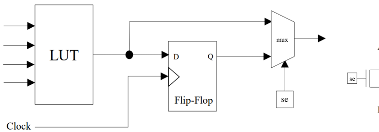
Figure 2. Structure of Configurable Logic Block (Temür 2013)
